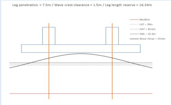
LEG LENGTH RESERVE & WAVE CLEARANCE
