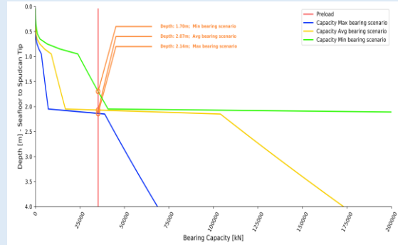
LEG PENETRATION & BEARING CAPACITY
