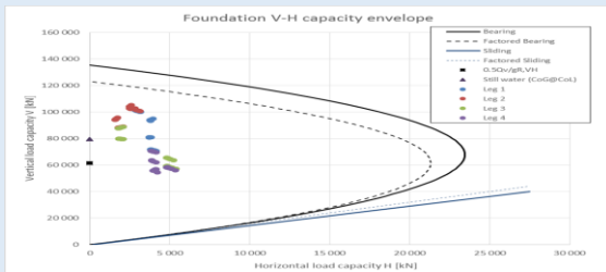
SOIL CAPACITY CURVE
