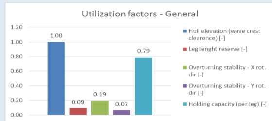
JACK-UP UTILIZATION FACTORS
